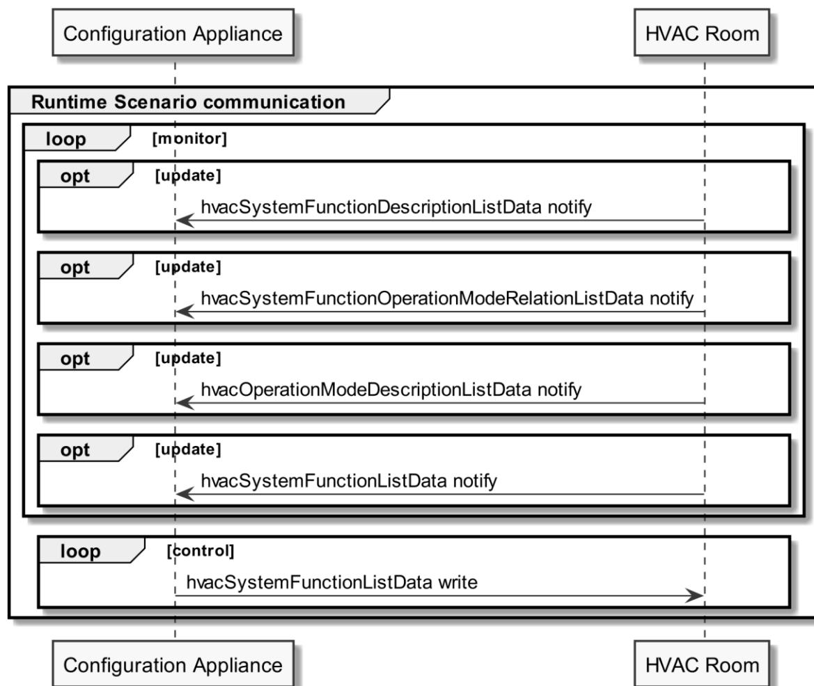
882 Figure 10: Scenario 1 - Runtime Scenario communication sequence diagram
